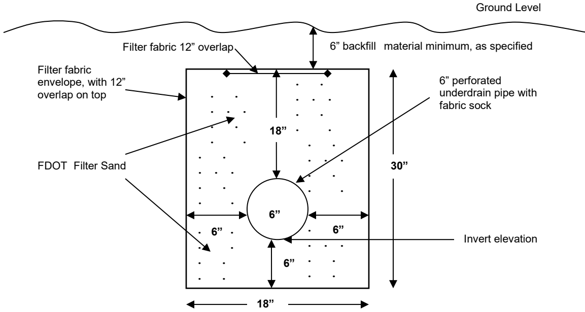
Typical Detail for 6" Pipe
