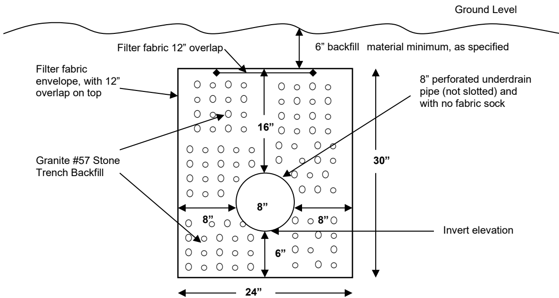
Typical Detail for 8" Pipe
